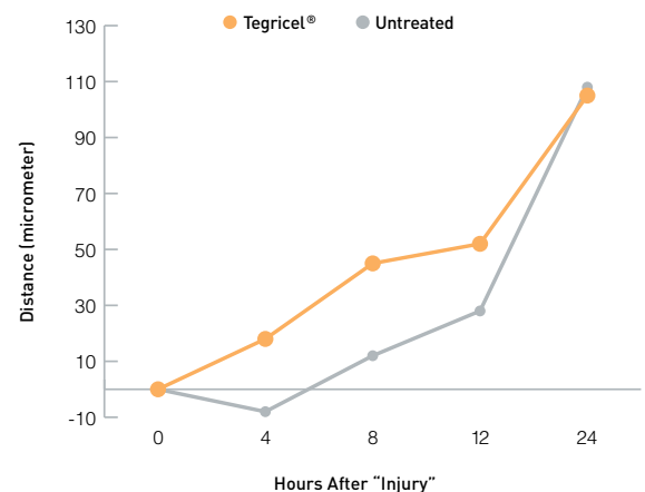
Healing of "Wound" by Migrating Gut Epithelial Cells
