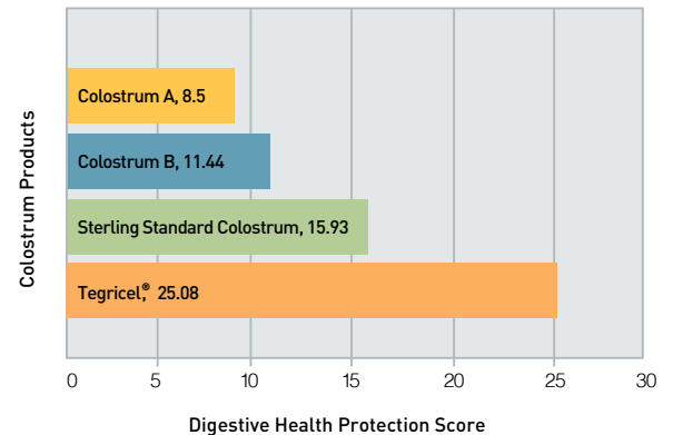
Cell Culture Analysis
